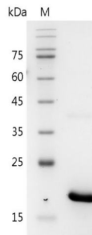
SDS-PAGE analysis of recombinant mouse IL-17B
